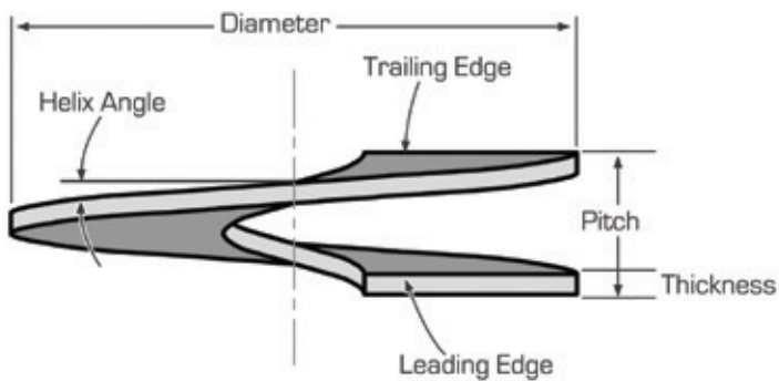
Figure 2: Helix Plate Geometry
