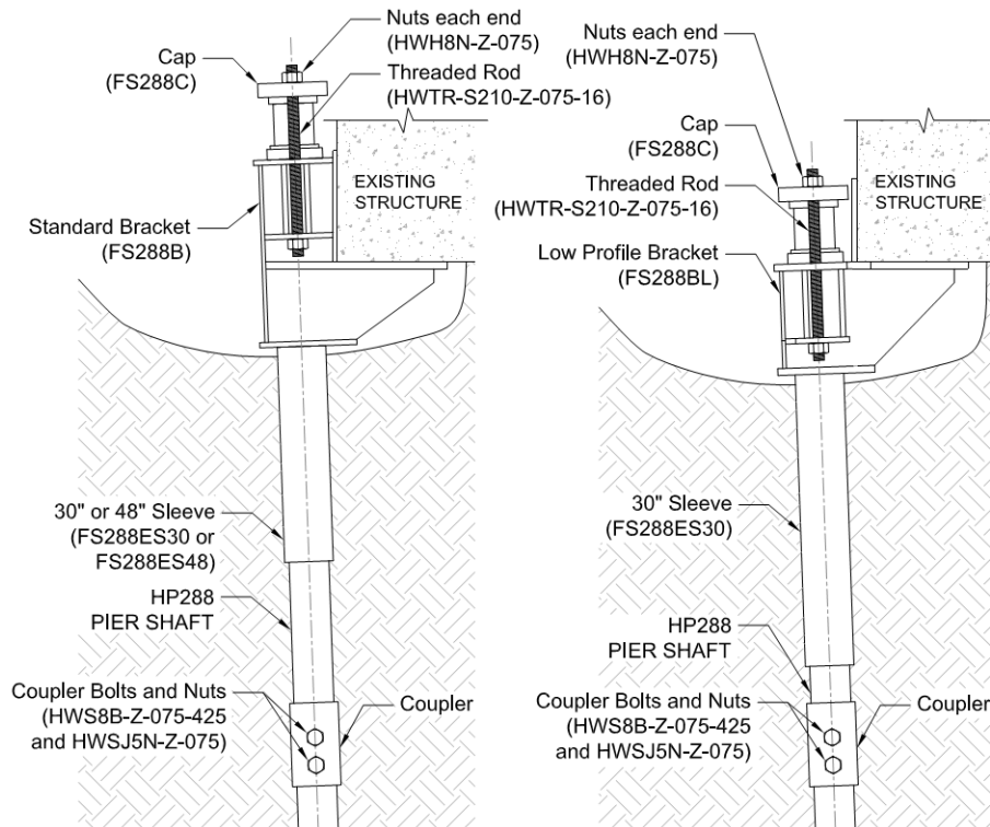
FIGURE 1—HP288 RETROFIT BRACKET AND SHAFT ASSEMBLIES
