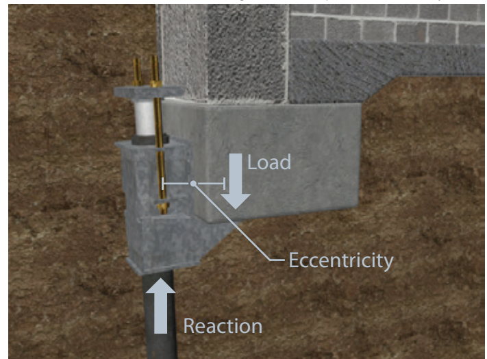
Figure 2: Retrofit piers are eccentrically loaded.
